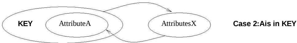
Transitive Dependencies
